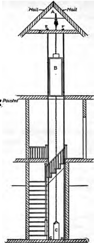
FIG. 228. — Front View of Elevator-Shaft and Stairs.
